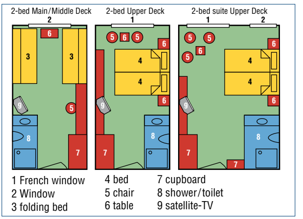
A typical 2-bed Upper Deck cabin
